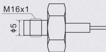
350S Pressure Transducer
